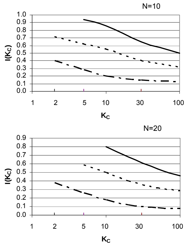
Figure 6-15 Interaction factor I versus K_C -number for N = 10 , N = 20 and different values of S/D . Solid curve: S/D_b = 2.88 . Dotted curve: S/D_b = 1.44 . Dash-dotted curve S/D_b = 0.87 .
