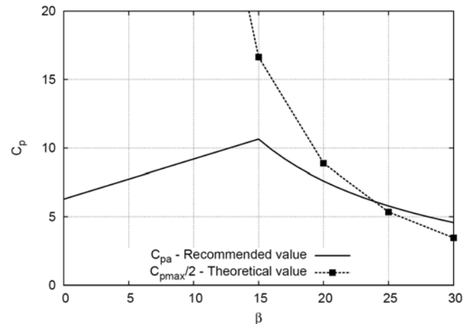
Figure 8-10 Space average slamming pressure coefficient C_{Pa} compared with C_{Pmax}/2 from Table 8-1 for a wedge shaped body as a function of local deadrise angle \beta .
