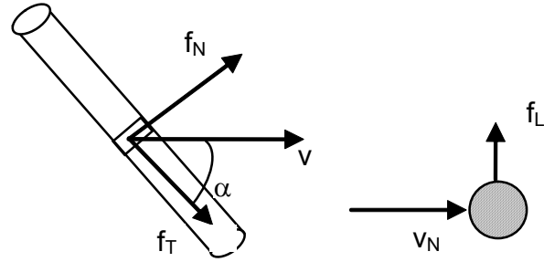
Figure 6-1 Definition of normal force, tangential force and lift force on slender structure.
